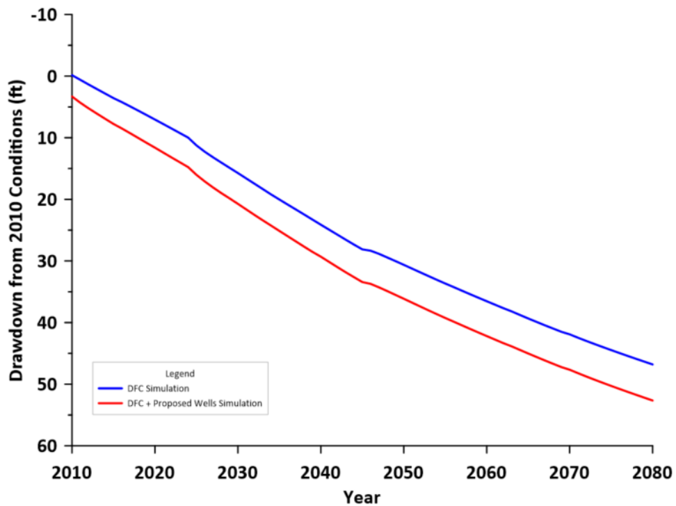
HAGM Drawdown (Evangeline) Layer 1, Row 33, Column 95 (BWLL-4025)
