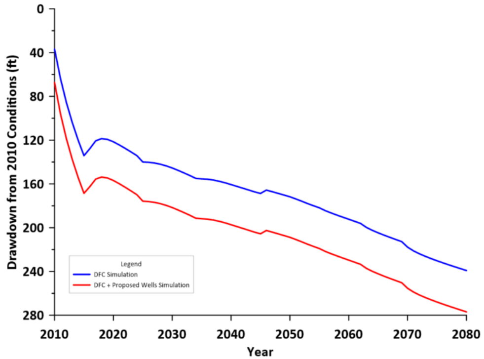
HAGM Drawdown (Jasper) Layer 1, Row 33, Column 96 (Woodhaven 1 and 2 Site)
