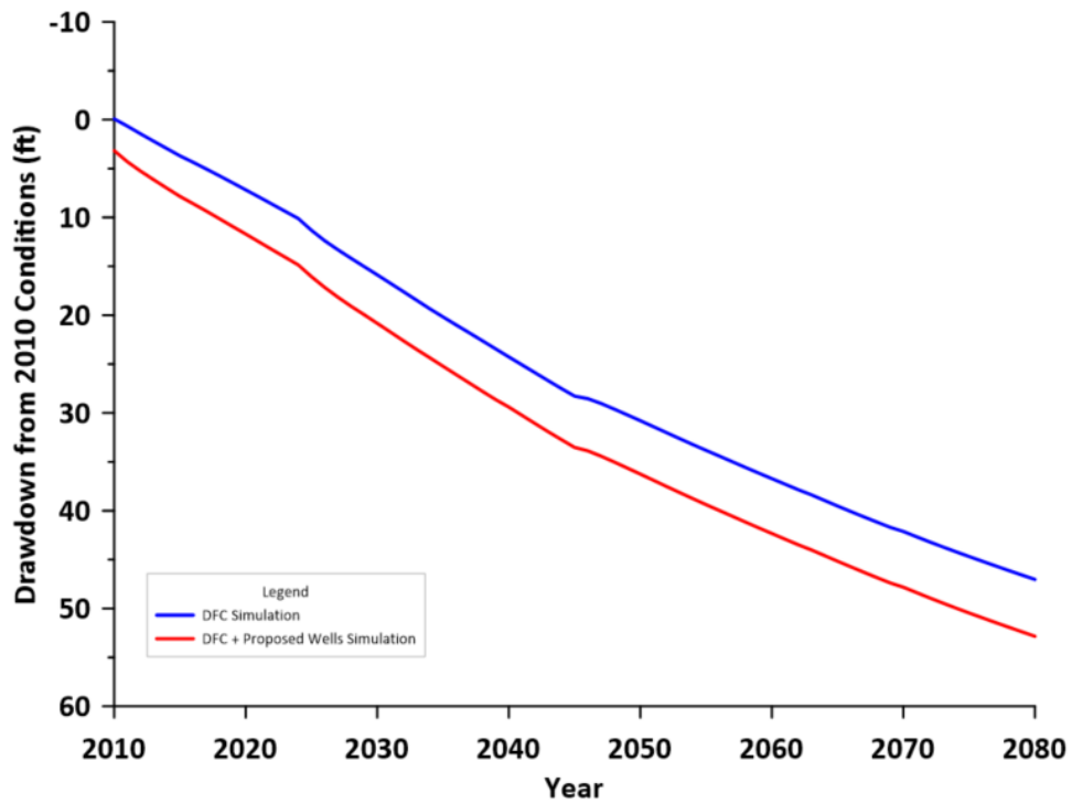
HAGM Drawdown (Burkeville) Layer 1, Row 33, Column 95 (BWLL-4025)
