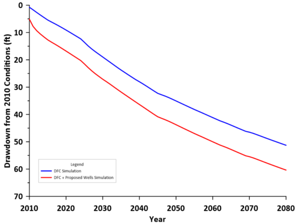
HAGM Drawdown (Burkeville) Layer 1, Row 33, Column 96 (Woodhaven 1 and 2 Site)
