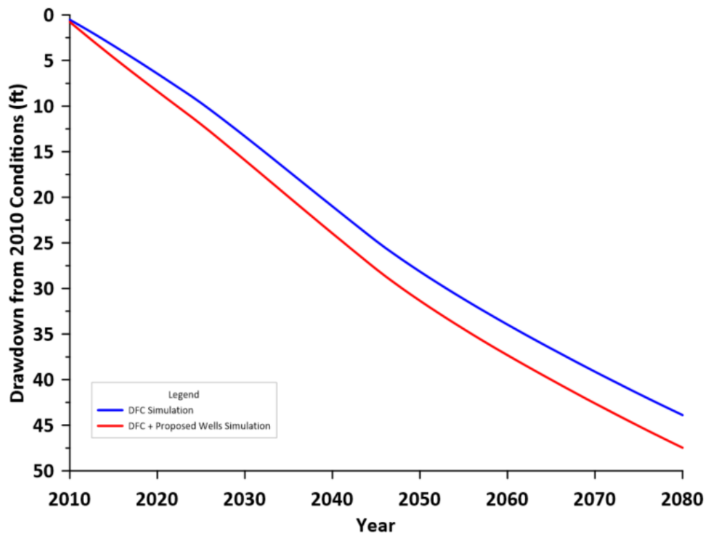
HAGM Drawdown (Chicot) Layer 1, Row 33, Column 95 (BWLL-4025)
