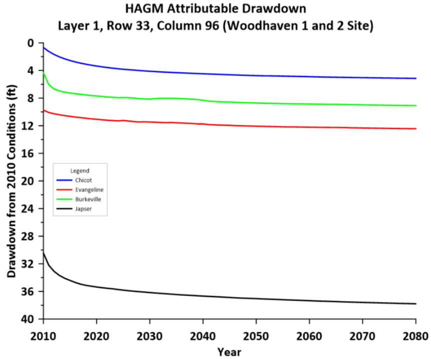
Figure 2. Attributable Drawdown Hydrograph for Woodhaven Well Sites
