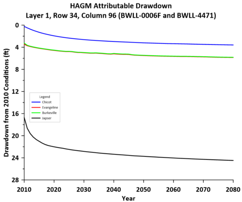
Figure 3. Attributable Drawdown Hydrograph for BWLL-0006F and BWLL-4471 Sites
